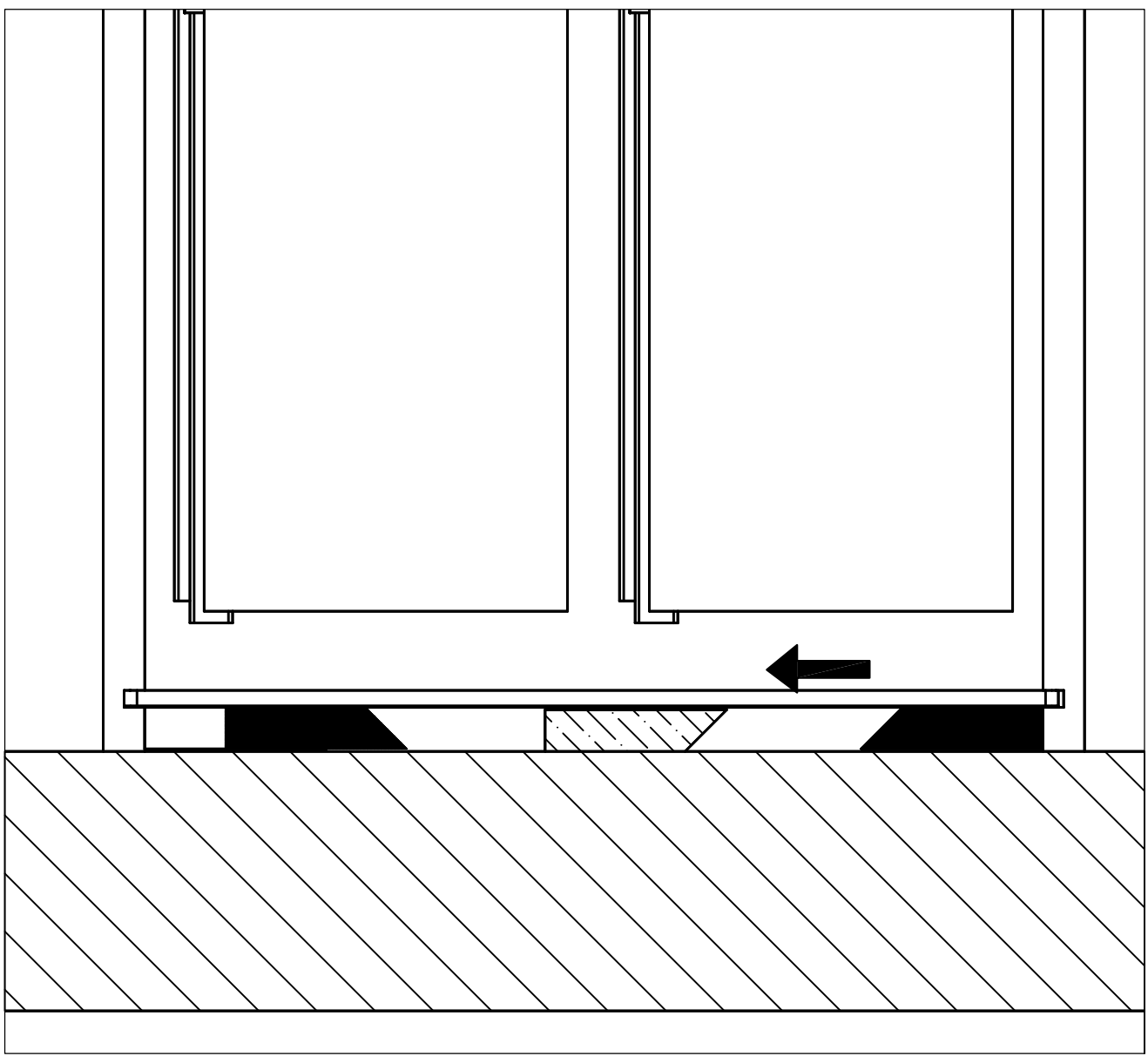
Montage air-6714-6728
